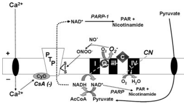
Fig. 3. Oxidative stress-initiated metabolism of mitochondrial NAD by PARP-1. Inhibition of mitochondrial respiration by cyanide (CN) stimulates production of superoxide ( O_2^- ), which reacts with nitric oxide ( NO ), forming peroxynitrite ( ONOO^- ). In the absence of reducing power to maintain sulfhydryl groups in a reduced redox state, peroxynitrite leads to net sulfhydryl oxidation. This oxidized redox state together with elevated intramitochondrial Ca^{2+} results in activation of the cyclophilin D (CyD)-dependent and cyclosporin A (CsA)-inhibitable permeability transition pore (PTP). Release of mitochondrial pyridine nucleotides through the PTP promotes further NAD metabolism by cytosolic/nuclear PARP-1. Activation of mitochondrial PARP may also contribute to NAD degradation. The presence of either exogenous or endogenous pyruvate helps to maintain a reduced mitochondrial redox state, thereby conferring protection against both PTP and PARP-1 activation.
