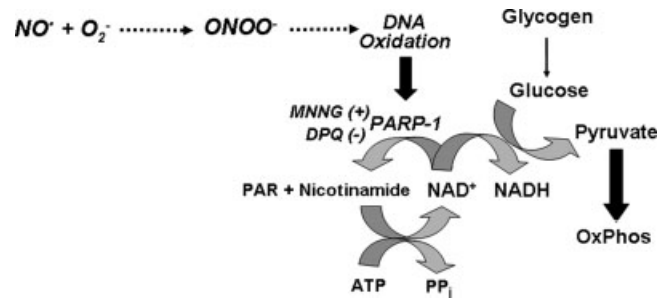
Fig. 1. Oxidative stress-initiated metabolism of cytosolic NAD by PARP-1. Superoxide ( O_2^{\cdot-} ), produced from mitochondria and other sources, reacts with nitric oxide ( NO\cdot ), producing peroxynitrite ( ONOO^- ), a powerful oxidant of DNA and proteins. DNA oxidation activates poly(ADP-ribose) polymerase 1 (PARP-1), which metabolizes NAD to nicotinamide and poly(ADP-ribosylated) (PAR) proteins. The fall in NAD can inhibit the glycolytic production of pyruvate, a major source of fuel for oxidative phosphorylation (OxPhos). Resynthesis of NAD from nicotinamide is dependent on the energy supplied by ATP. PARP-1 can be alternatively activated by exposing cells to MNNG and inhibited by exposure to DPQ.
